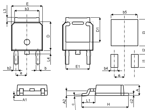
TO-252, (TO-252)
