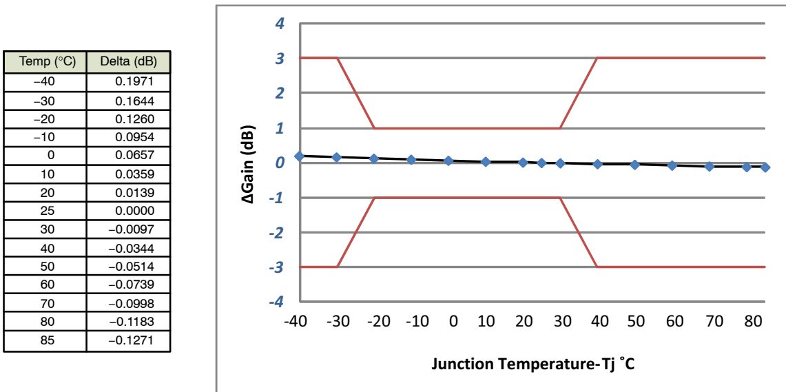
Figure 6. \Delta Gain vs. Temperature (Nominal Temperature = 25^\circ\text{C} )
