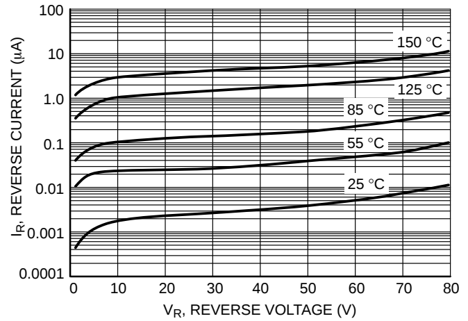
Figure 2. Reverse Current
