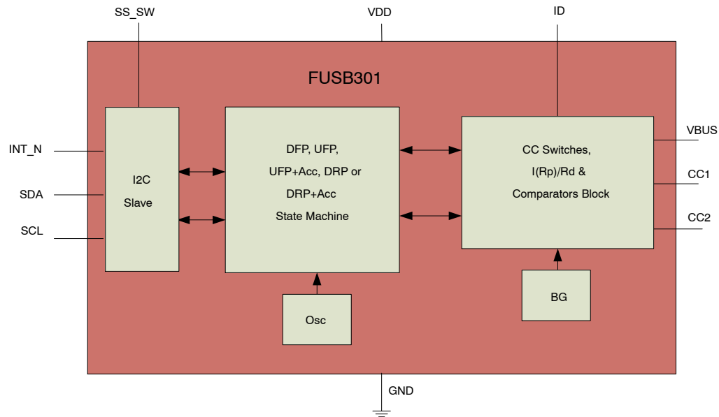
Figure 2. Block Diagram
