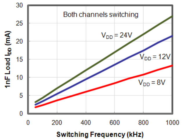
Figure 10. I_{DD} (1 nF Load) vs. Frequency
