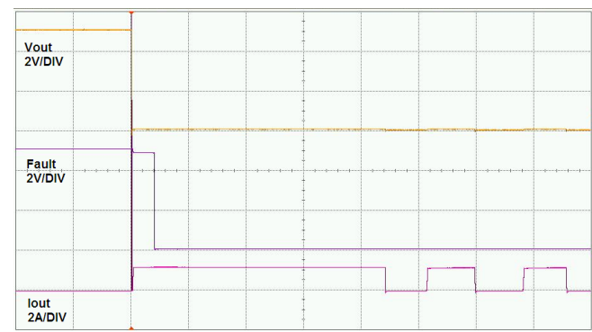
Figure 8. Extended Short-Circuit into Thermal Cycles
