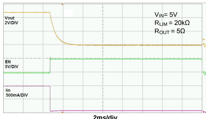
Figure 4. Turn-Off Delay and Fall Time
